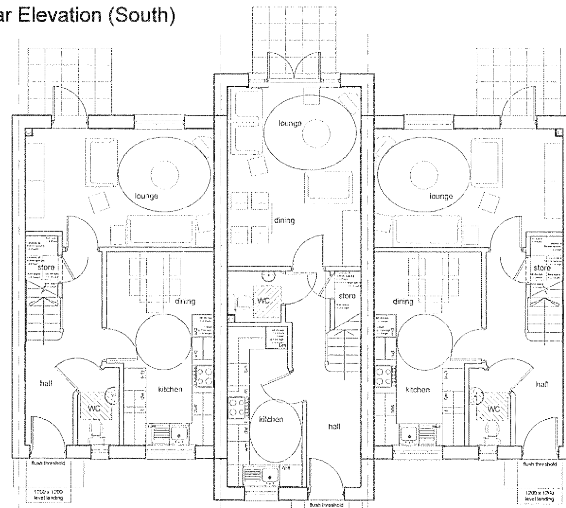
Type 10 3 - Bedroom House Ground Floor Plans
