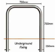
Cycle stand fixing
