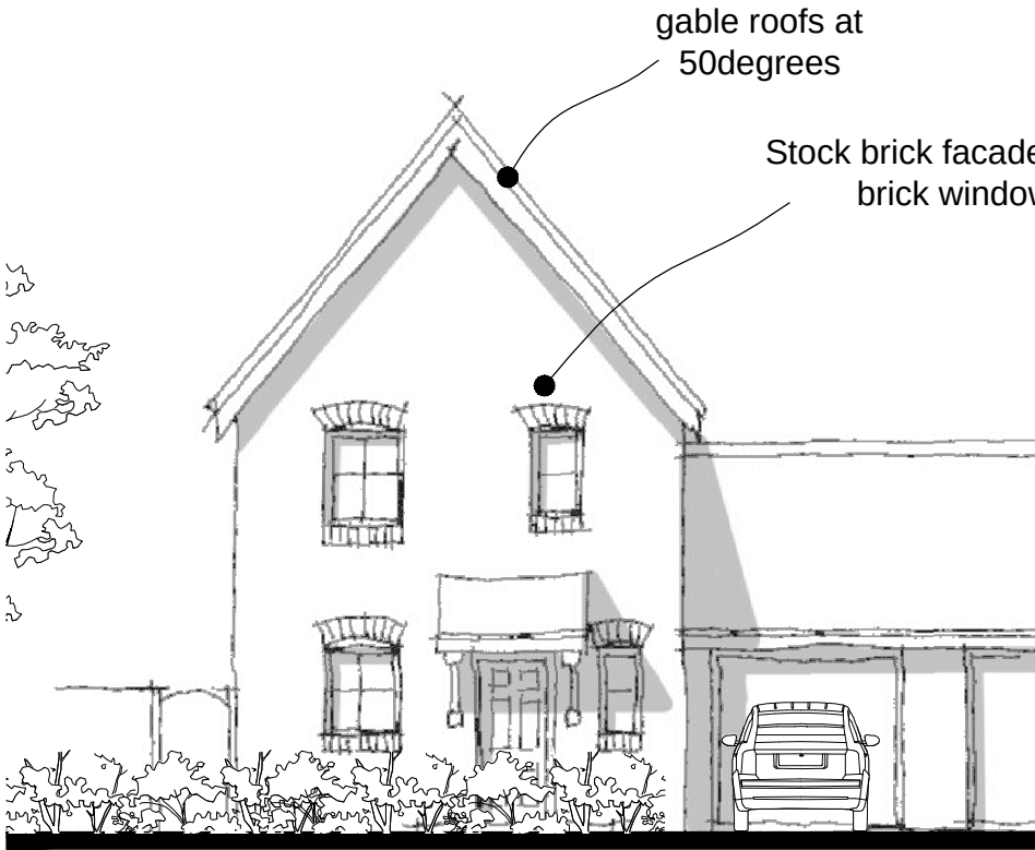
Front Elevation (North)
