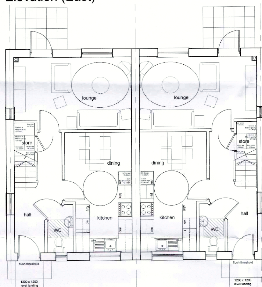
Plot 18 3 - Bedroom House
