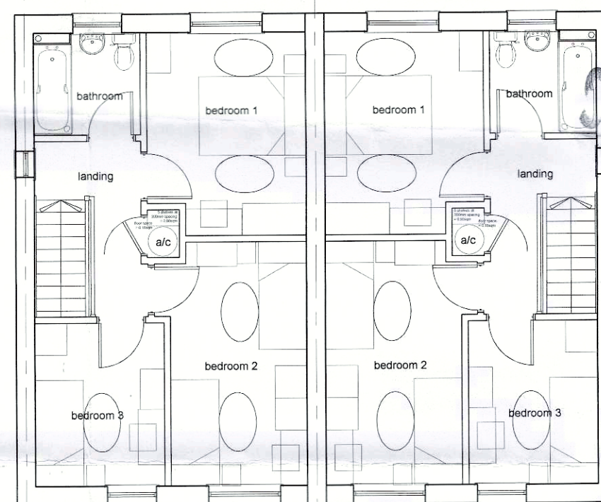
First Floor Plans
