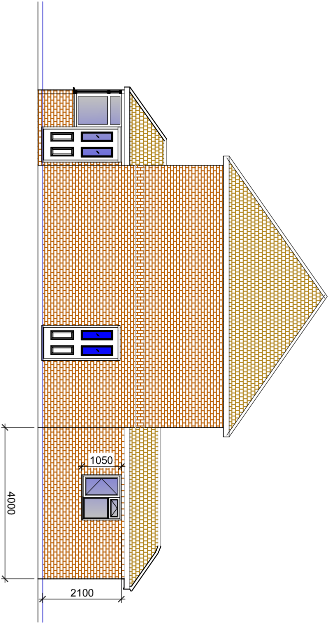
SIDE ELEVATION - EAST PROPOSED
