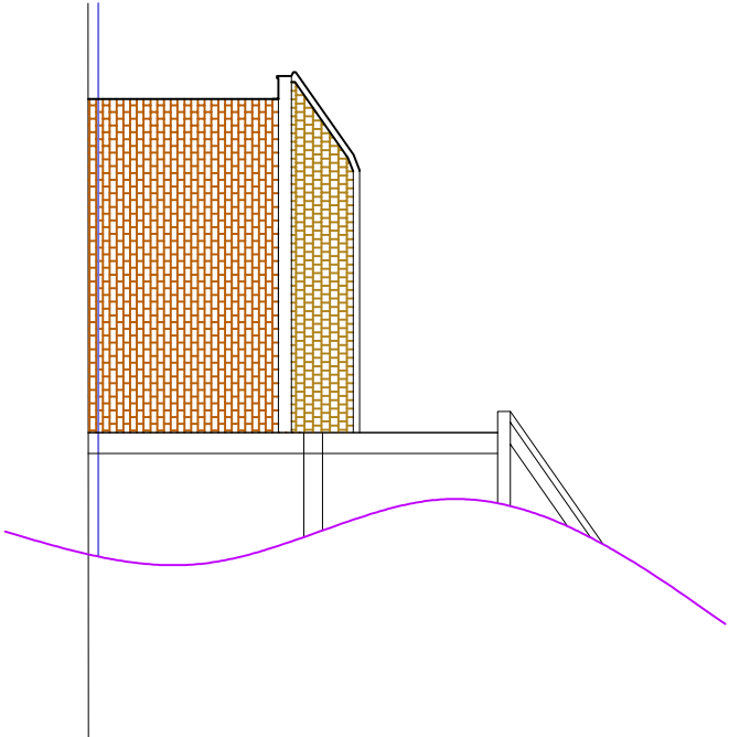
SIDE ELEVATION - WEST PROPOSED
