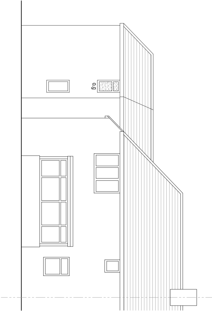
Rear Elevation (East) @ 1:100
