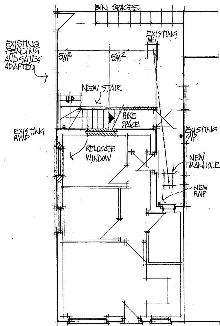
GROUND FLOOR PLAN-EXISTING TWO BEDROOM FLAT
