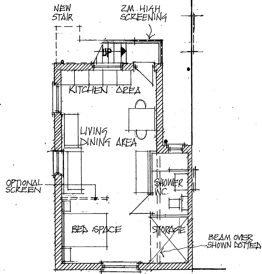
FIRST FLOOR PLAN-PROPOSED STUDIO FLAT
