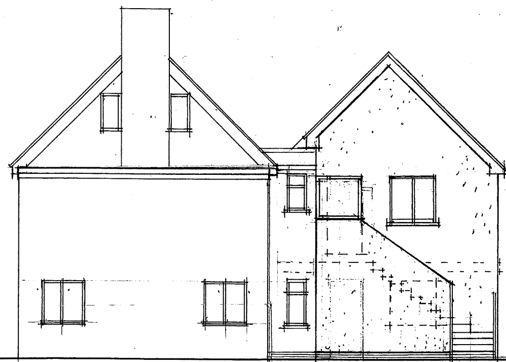
WEST ELEVATION
