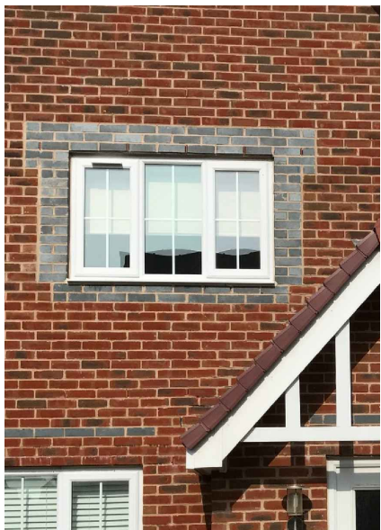
Brick detailing to windows 'constructed' image
