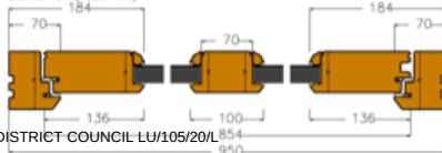
Section C1 (scale 1:4)
