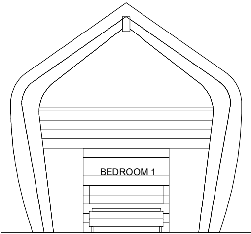
SECTION LOOKING EAST 1 1 : 100
