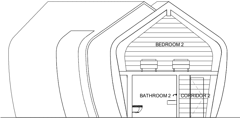
SECTION LOOKING EAST 2 1 : 100
