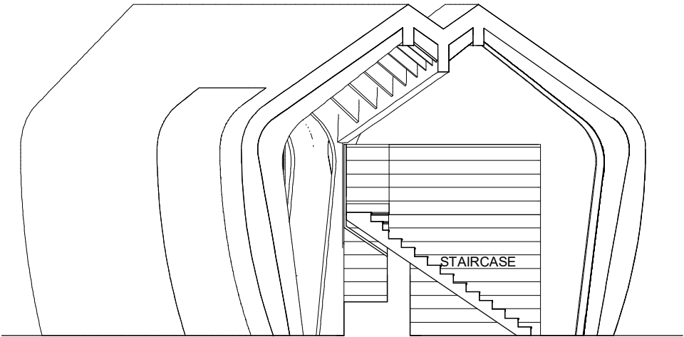
SECTION LOOKING EAST 3 1 : 100
