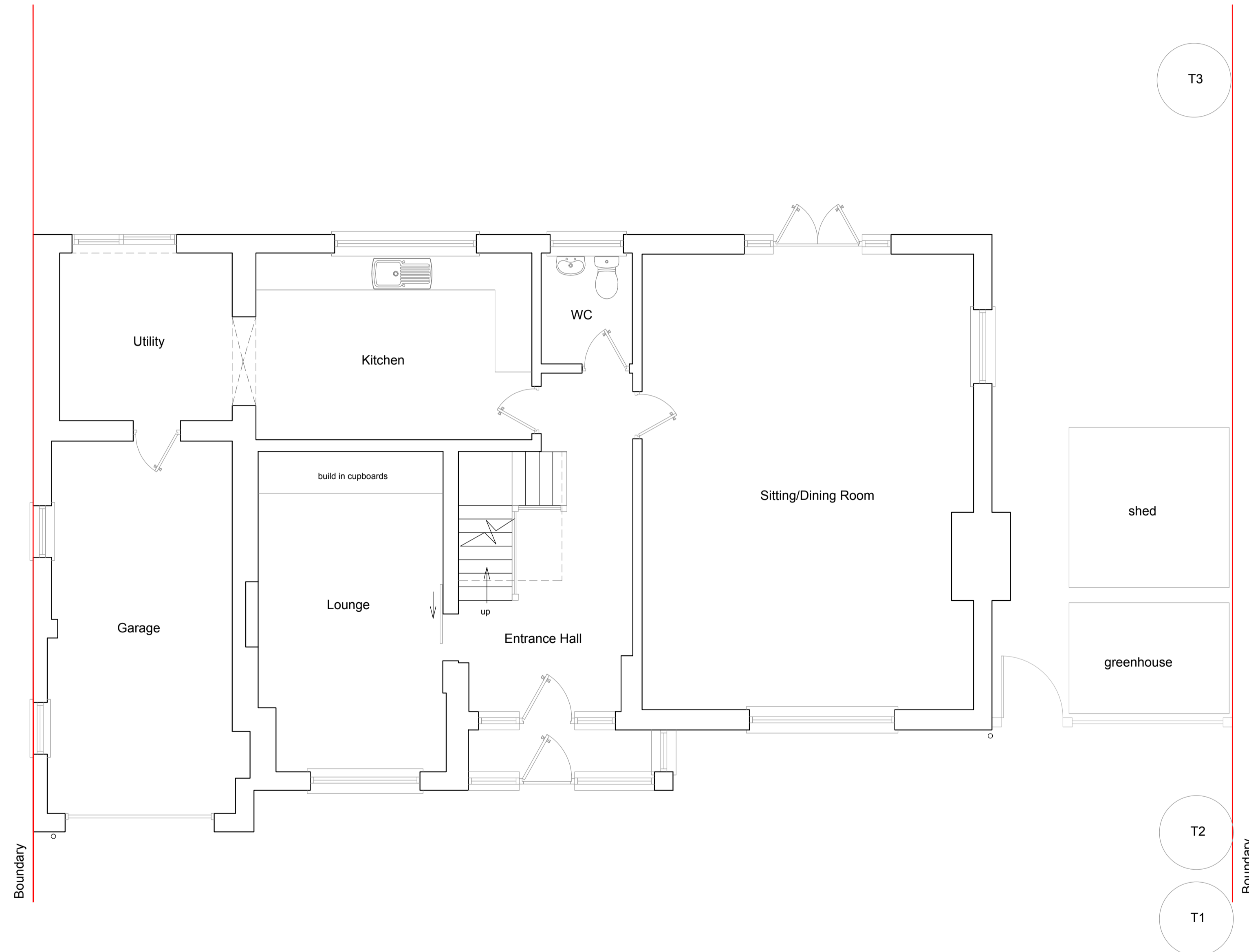
Ground Floor Plan Existing 1:50
