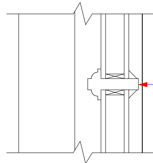
Fixed glazing bar ovolo profile
