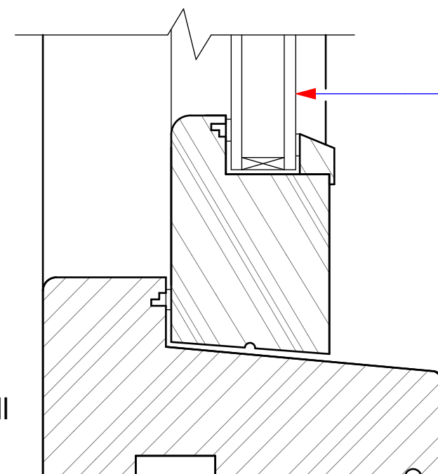
Vertical section
