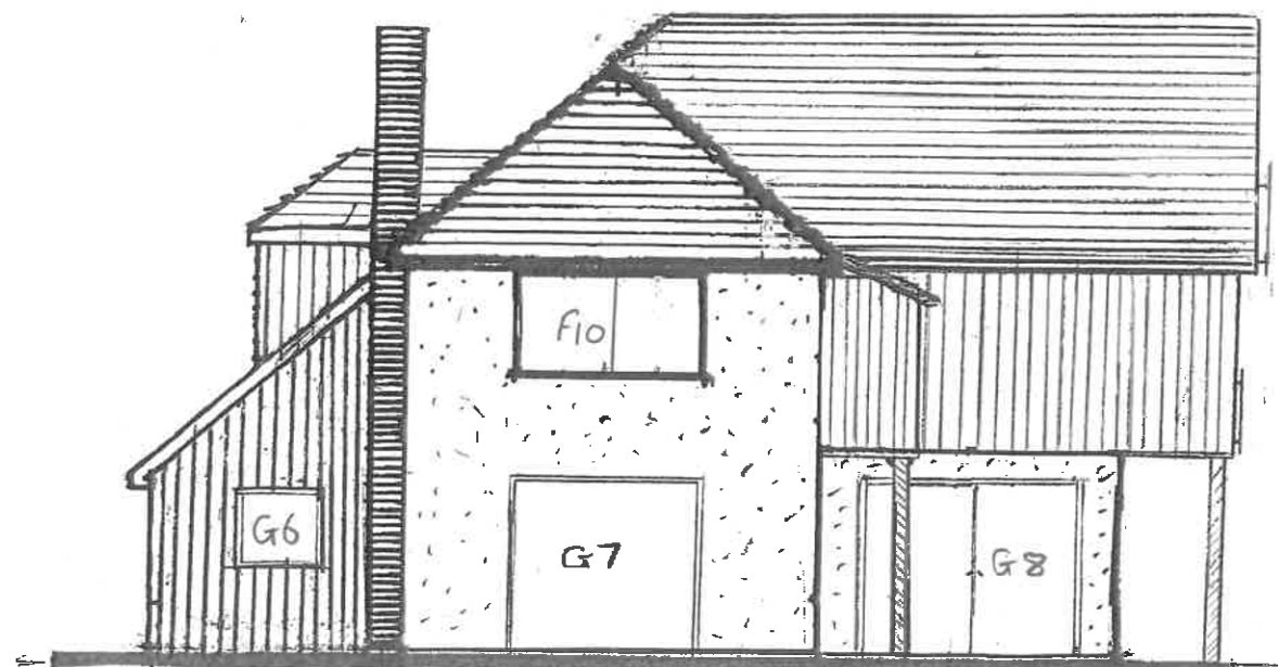
West Elevation
