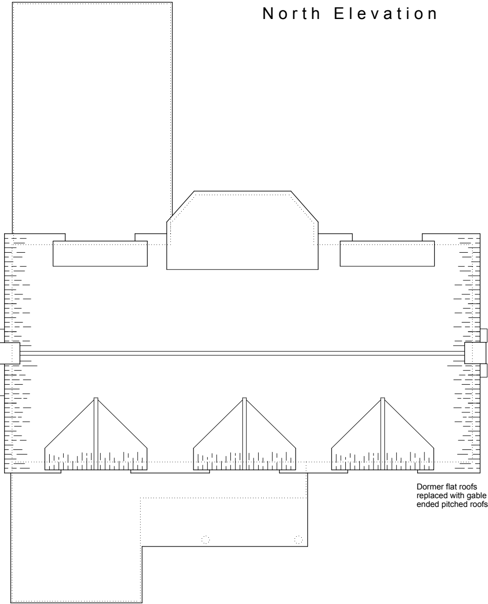
Roof Plan
