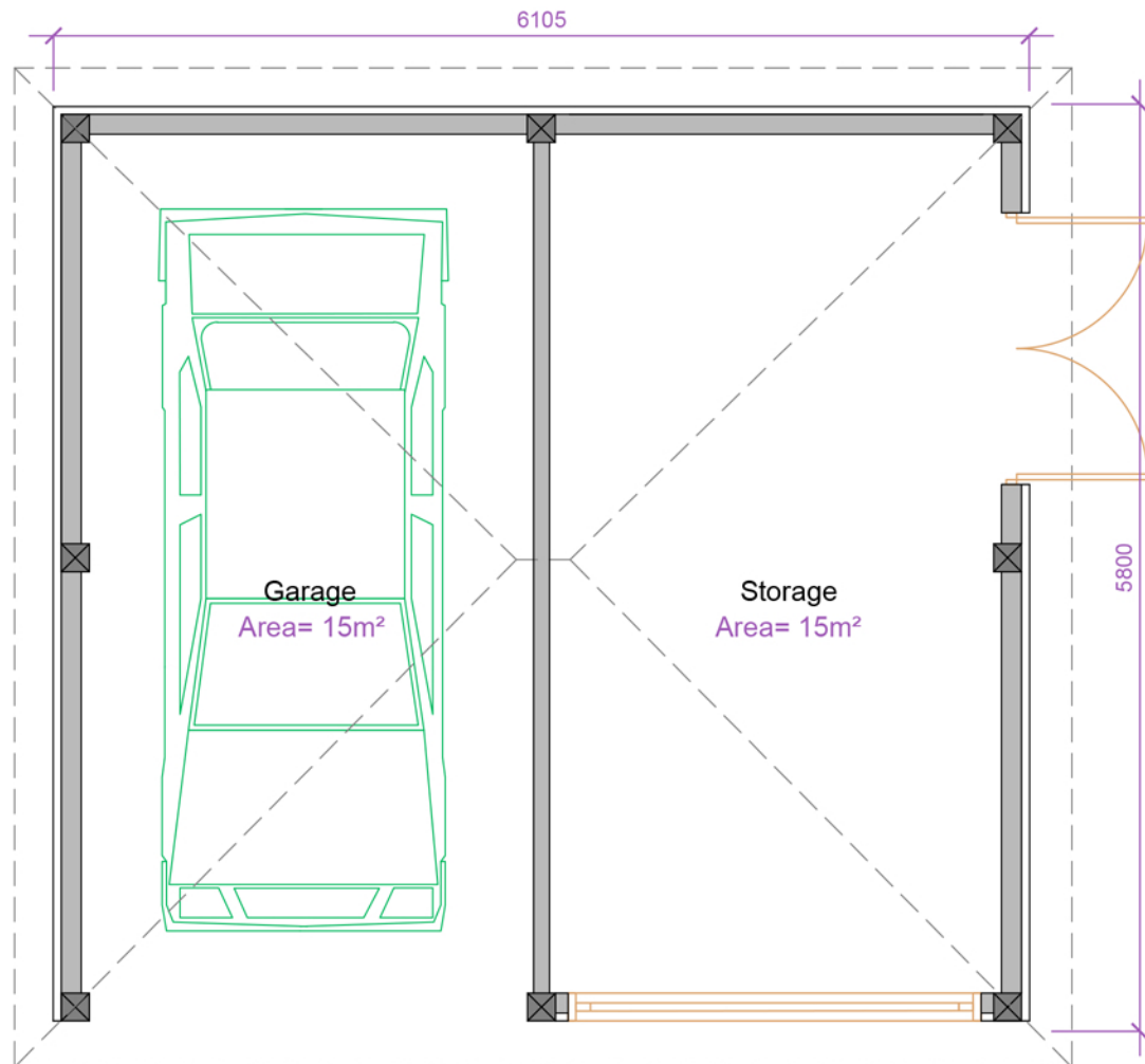
Floor Plan 1:50
