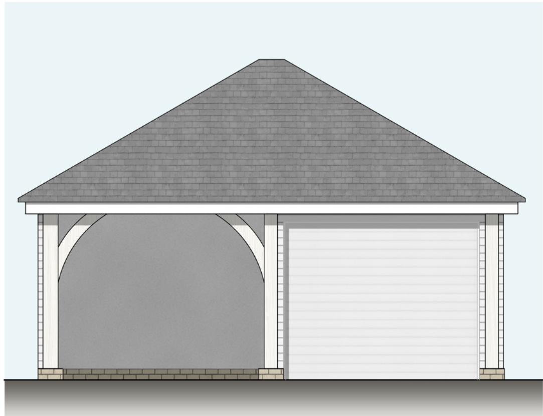
Front Elevation (South) 1:50
