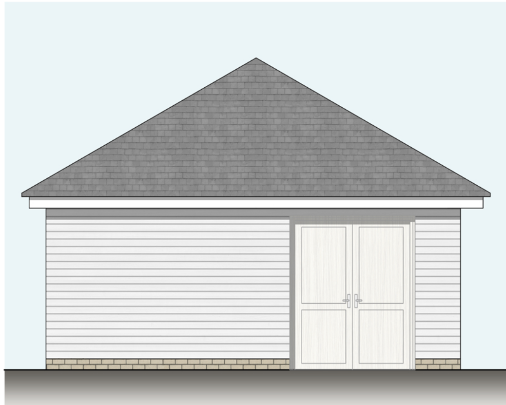
Side Elevation (East) 1:50
