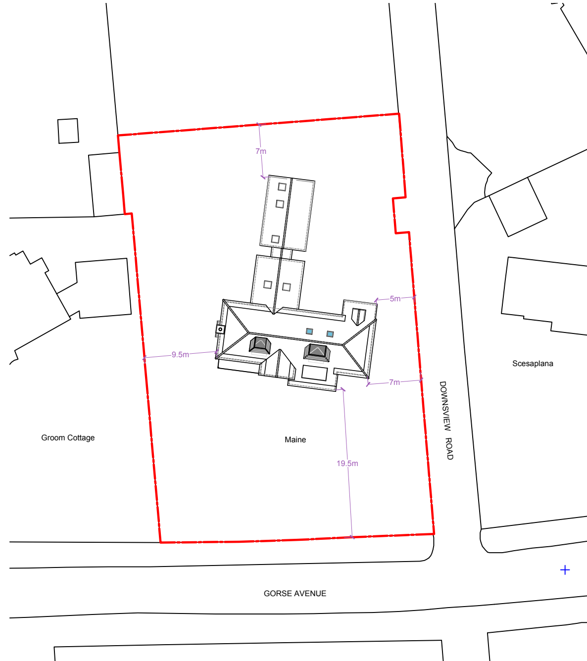
Block Plan 1:500
