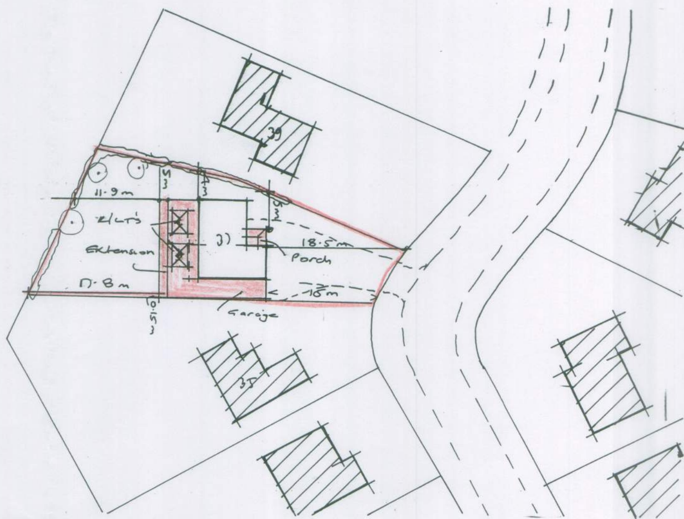
Block plan 1:500
