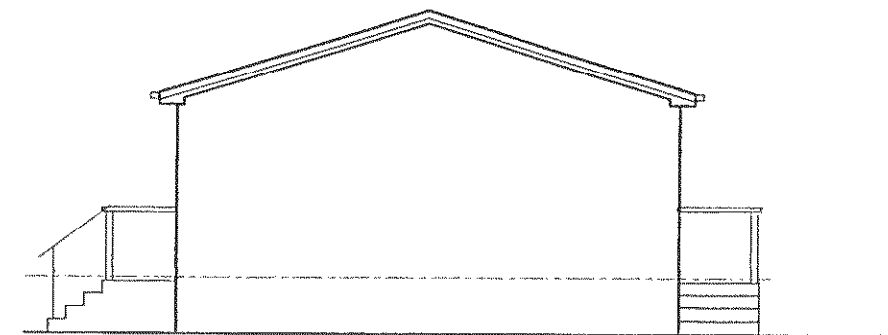
SOUTH ELEVATION
