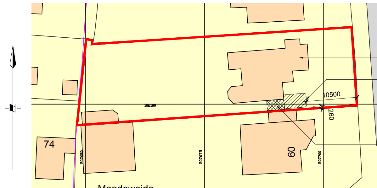
Proposed Site / Block plan 1:500 @ A3
