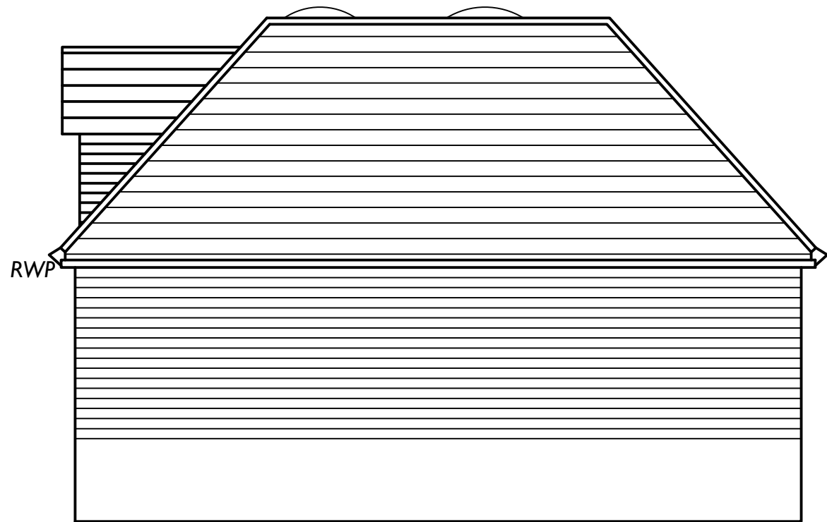
SIDE ELEVATION - EAST FACING
