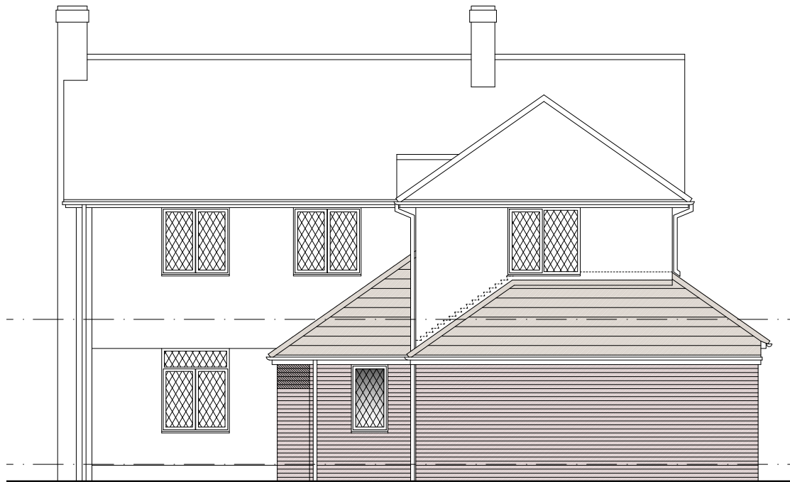
Proposed East Elevation (front) 1:100 @ A3
