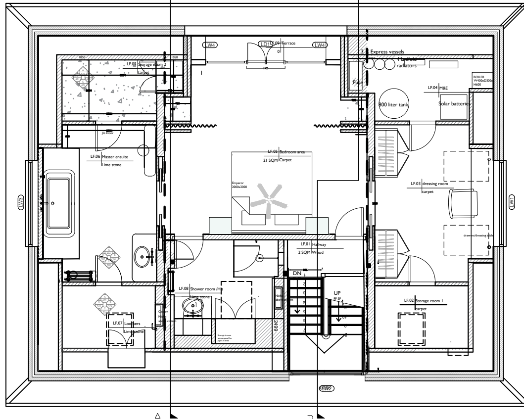
EXISTING SECOND FLOOR PLAN 1:50
