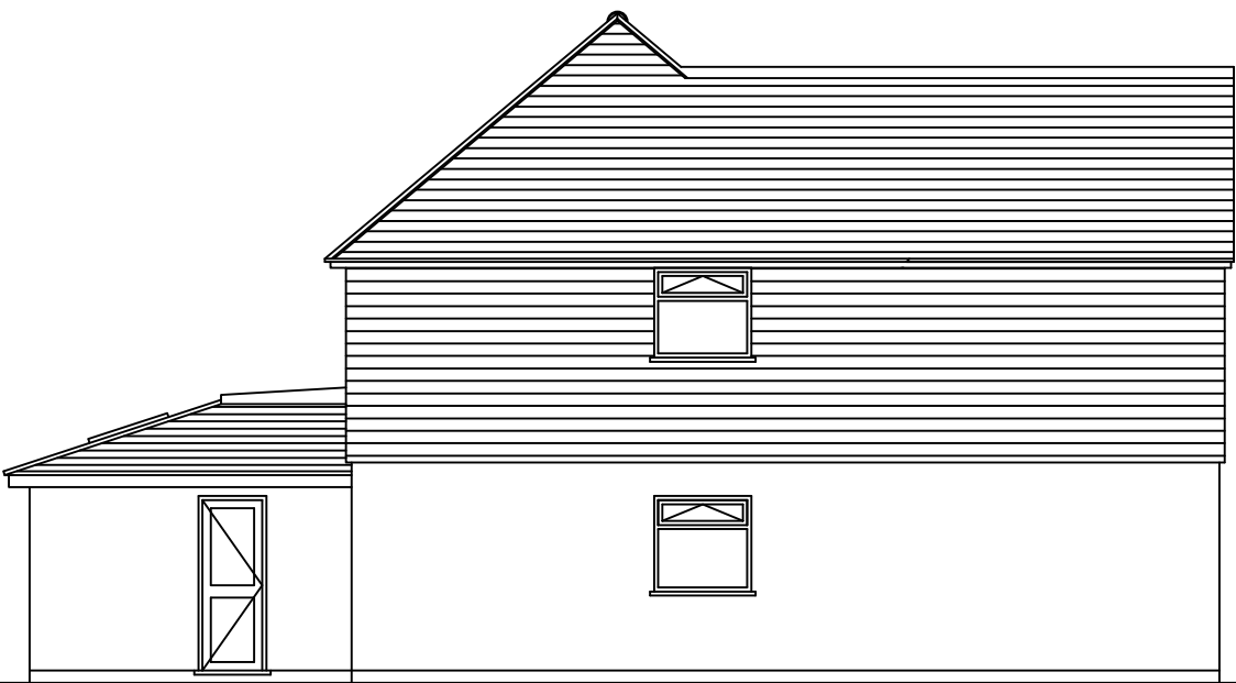
Proposed North East Elevation
