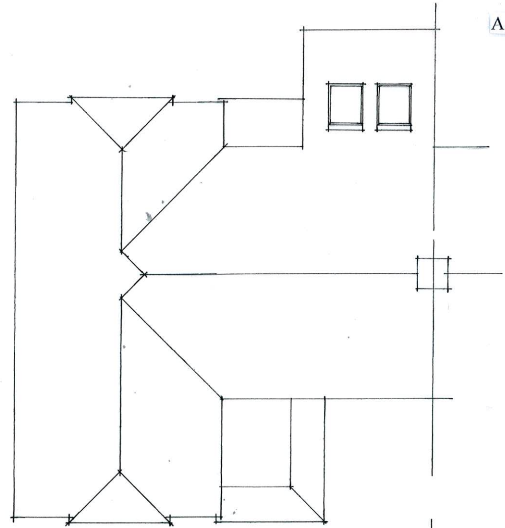
Existing Roof Plan 1/100
