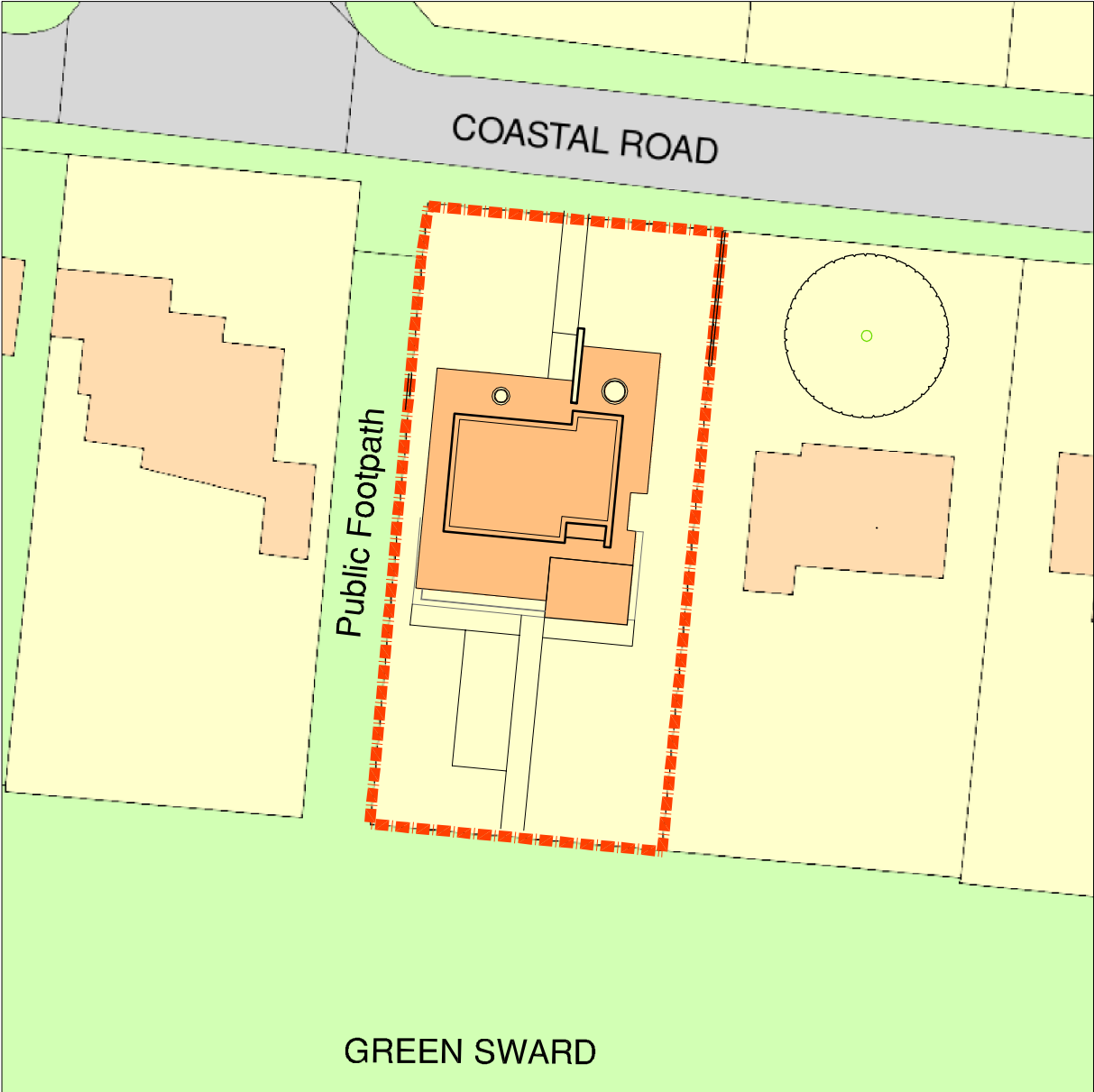
1:500 Block Plan as proposed
