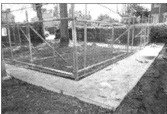
Photo 9: Plywood fixed to a wood frame is another effective method of protecting soil from pedestrian compaction.
