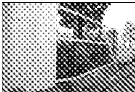
Photo 4: Board specification on secure wooden posts is a suitable alternative to the standard braced scaffold design.
