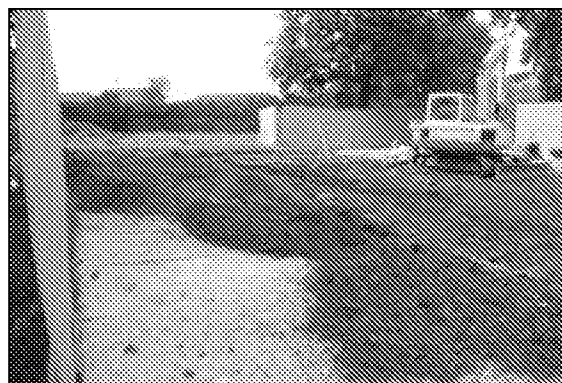
Photo 8: Spreading soil excavated from footings is an effective way of buffering the plywood surface from the wear of light vehicles.
