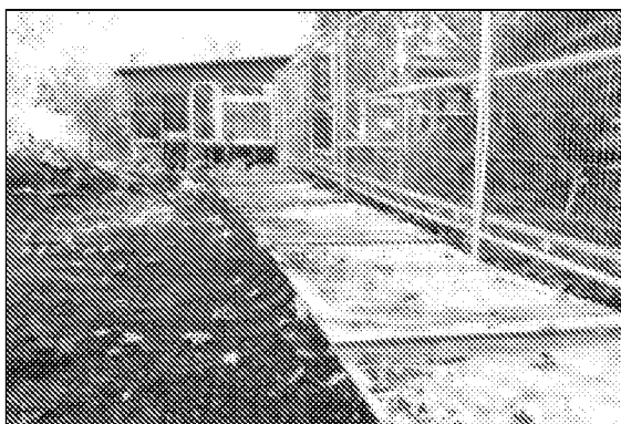
Photo 7: Heavy-duty plywood set onto a compressible woodchip layer and pinned into position is suitable to spread the loading from pedestrian access.
