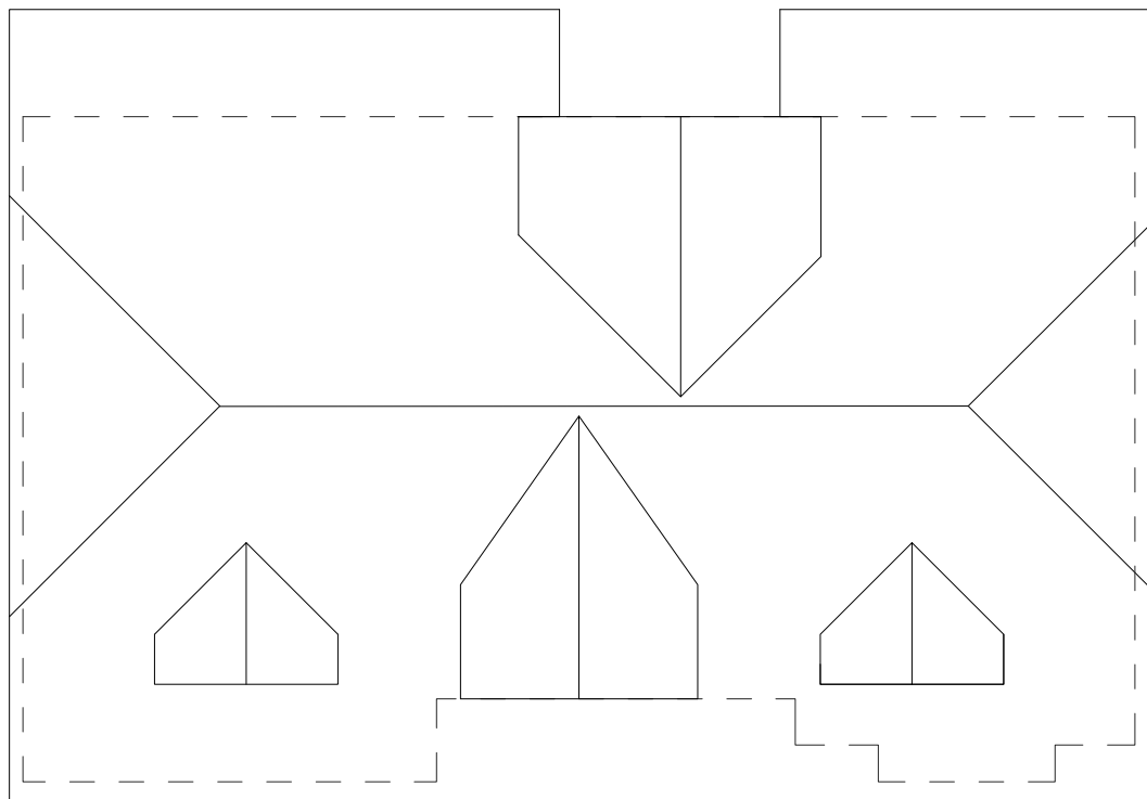
ROOF plan
