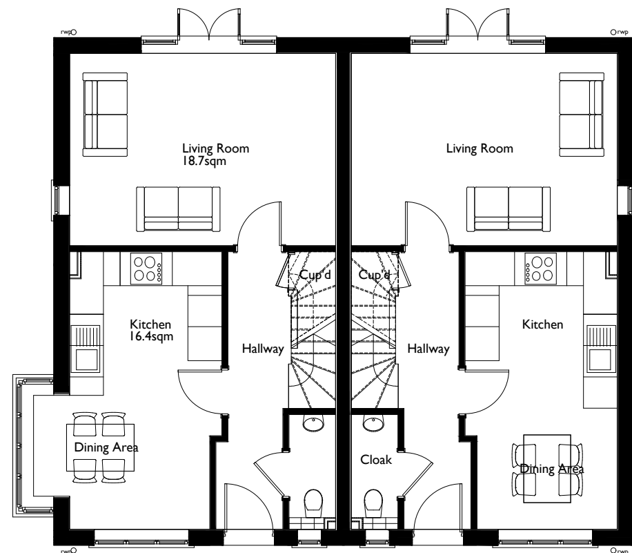
GROUND FLOOR PLAN Type E 3 Bedroom 2 storey house 92.0sq.m. / 982.0sq.ft. Plots 42-43
