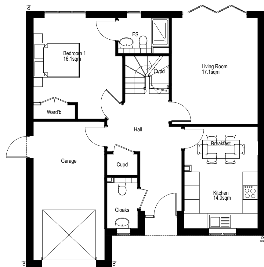
GROUND FLOOR PLAN Type B 3 Bedroom Chalet Bungalow. 130.0sq.m. / 1399.3 sq.ft. Plots 32
