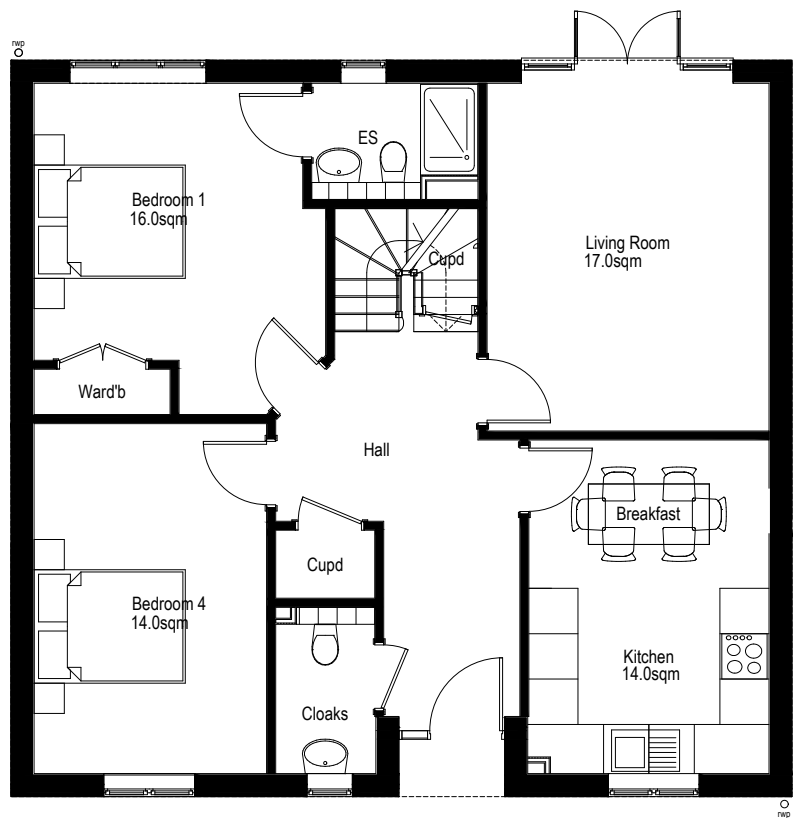
GROUND FLOOR PLAN Type A 3 Bedroom Chalet Bungalow. 148.0sq.m. / 1599.5 sq.ft. Plots 33
