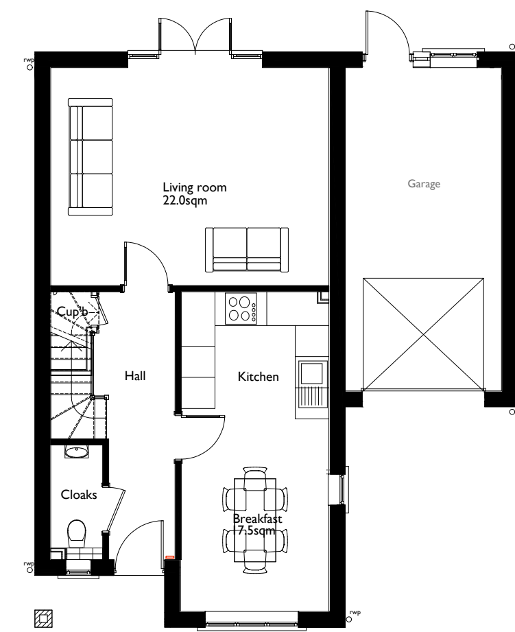
GROUND FLOOR PLAN Type H1 3 Bedroom 2 Storey House. 108.92sq.m. / 1172.41 sq.ft. Plots 1
