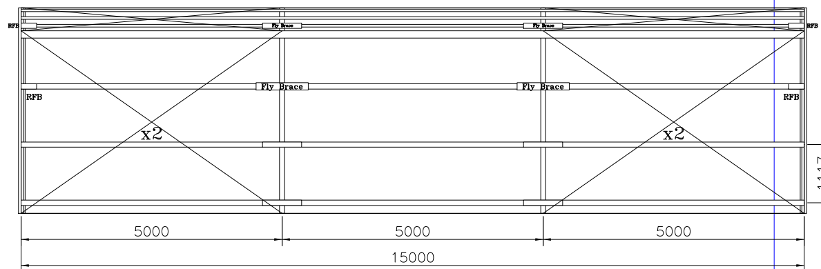
Left Elevation Frame (Scale = 1:100)
