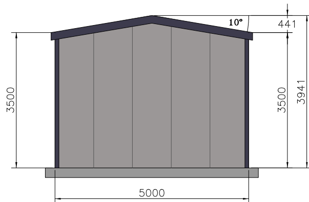
Front Elevation (External)
