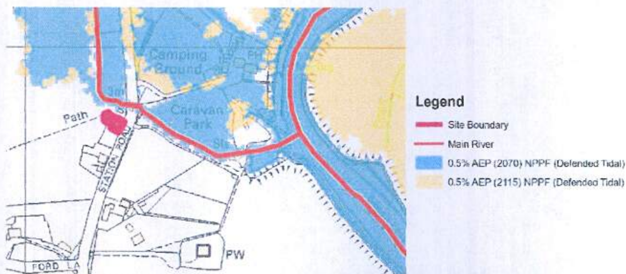
FIGURE 2.2.2.1 MODELLED FLOOD OUTLINE 0.5% AEP DEFENDED TIDAL
