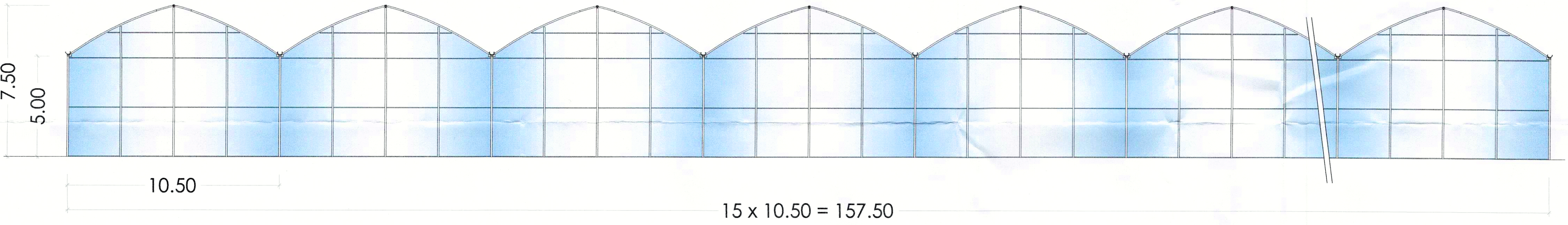
FRONT VIEW
