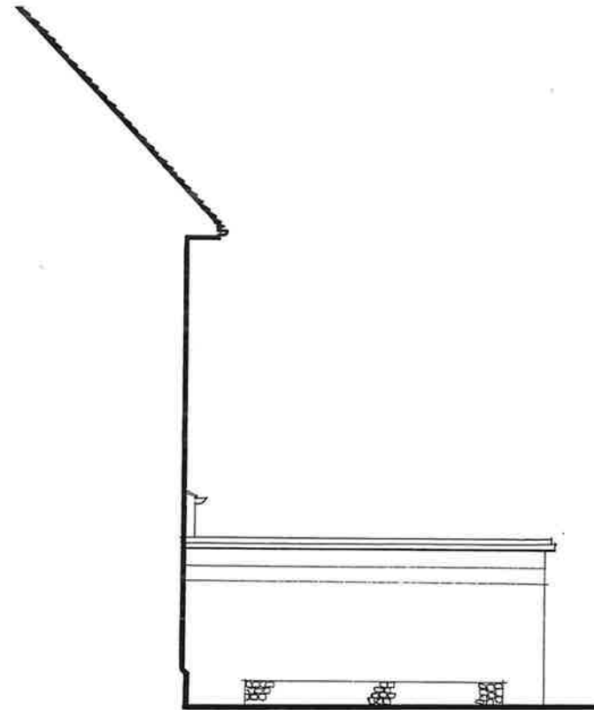
NORTH ELEVATION 1:100
