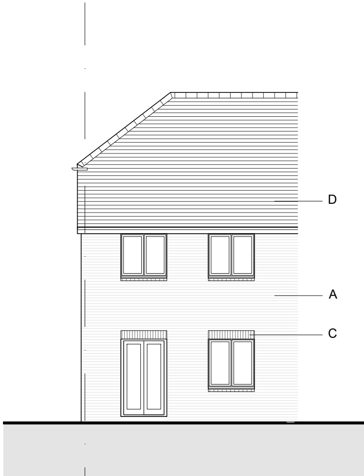
REAR elevation
