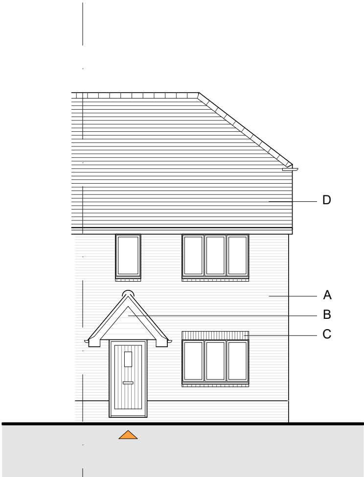
FRONT elevation
