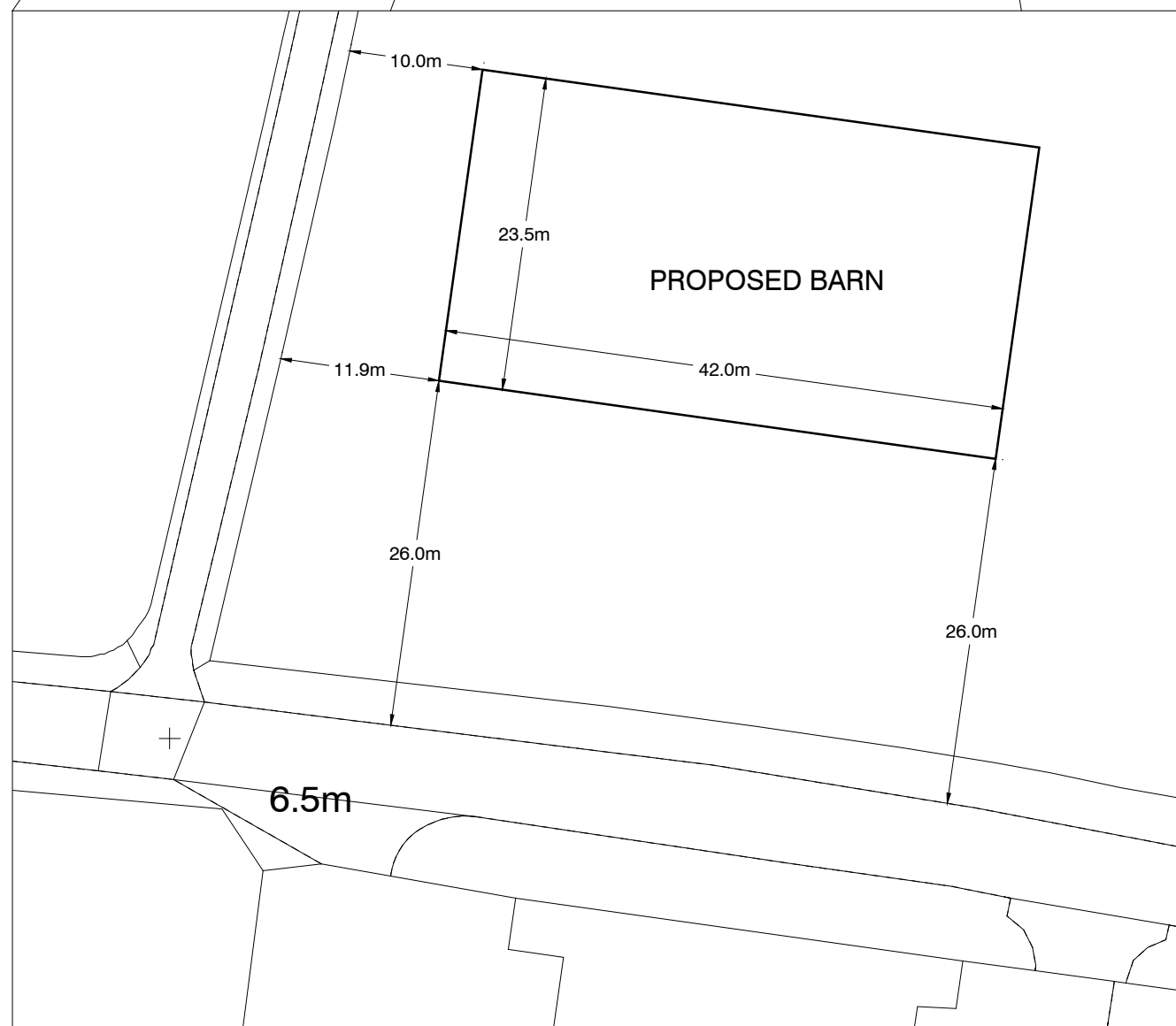
Block Plan 1:500@A1
