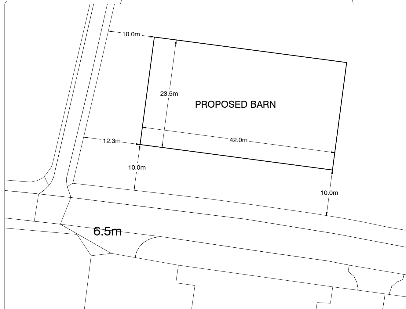
Block Plan 1:500@A1
