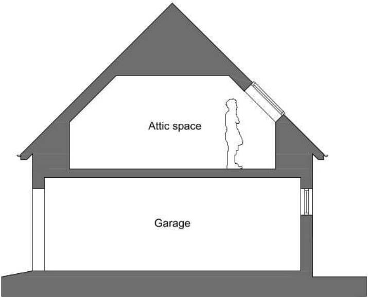
SECTION A
