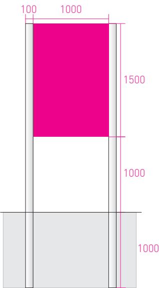
Stack Sign 1000x1500mm 100mm side mounted posts 1000mm ground clearance
