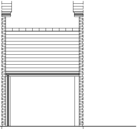
REAR ELEVATION
