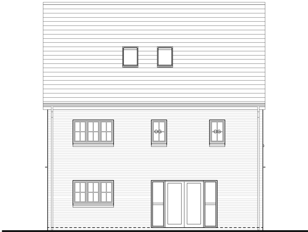
Rear Elevation
