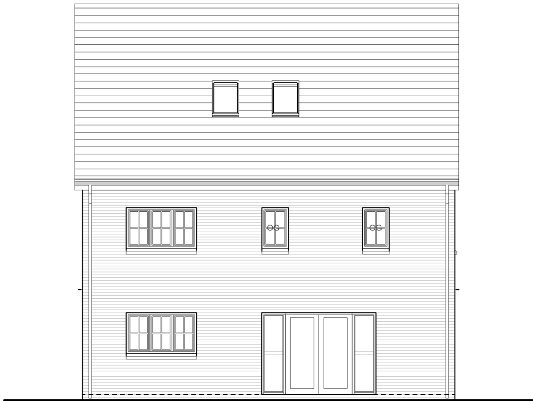
Rear Elevation
