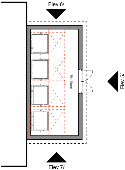
02 Floor Plan - Bin Store Type 2 Scale: 1:100
