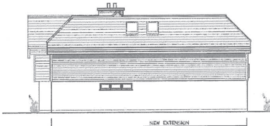
NORTH-EAST PROPOSED ELEVATION 1:100
