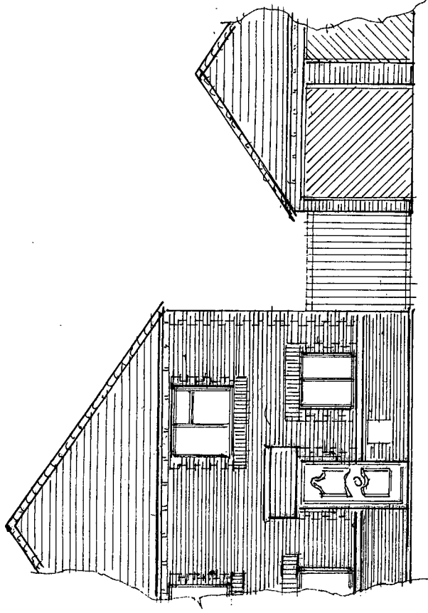
EXISTING EAST VIEW 1:100
