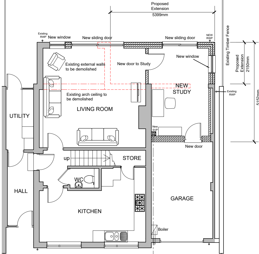
PROPOSED GROUND FLOOR PLAN PLAN B
