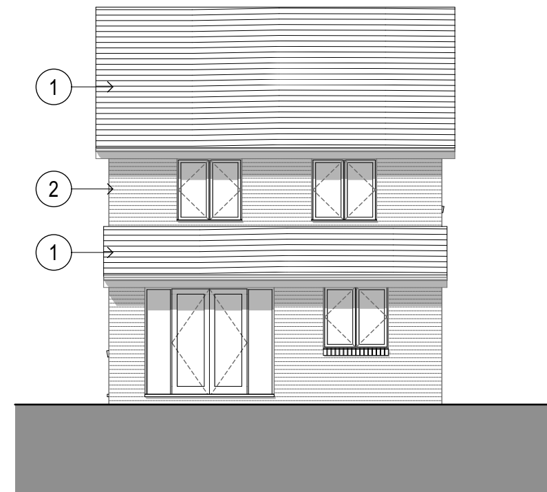
SIDE (NORTH WEST) ELEVATION 1:100
